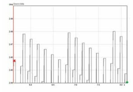
Figure 8: Frequency hopping in 2.4 GHz WLAN (FHSS).
