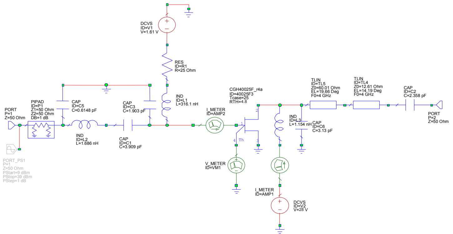
Figure 1 - 2 to 6 GHz, 25 W Broadband PA Schematic
