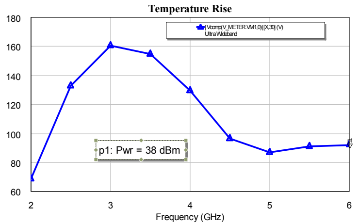
Figure 4 - Transistor temperature rise above T_{case} prior to optimization
